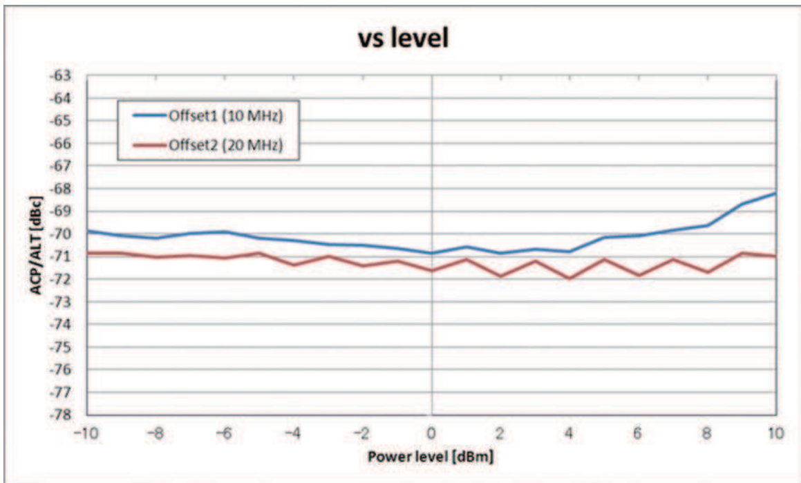
ACP/ALT vs. Power level (with MG3710A-041, Frequency: 2.1 GHz)
